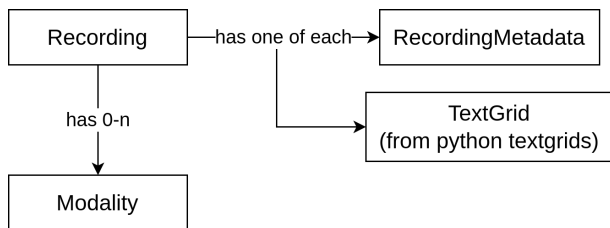
Figure 2: Recording class and its components.
